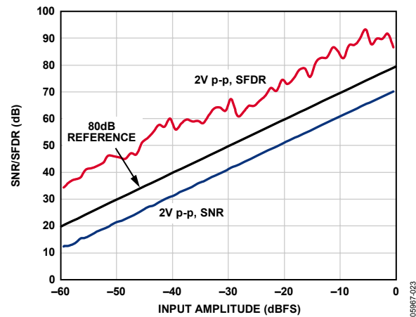
Figure 29. SNR/SFDR vs. Analog Input Level, f_{IN} = 10.3 MHz, AD9222-50
